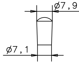
Toggle Switch Knopf toggle switch knobs
