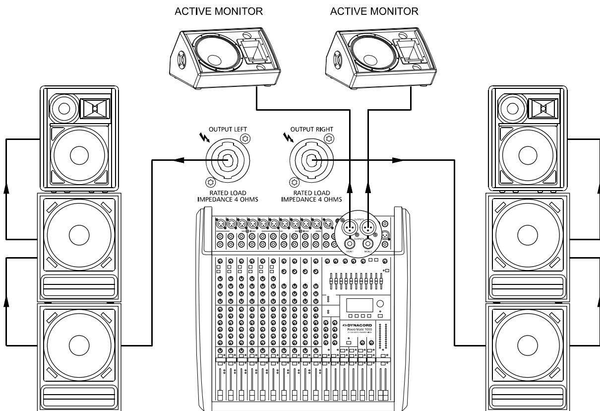
Illustration 6-1: Maximum amount of speakers in passive configuration
