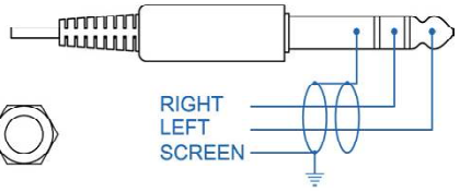
1/4" STEREO HEADPHONE JACK
