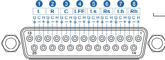
25 PIN D'SUB ANALOGUE IN/OUT wired to TASCAM's DB-25 Pinout Standard
