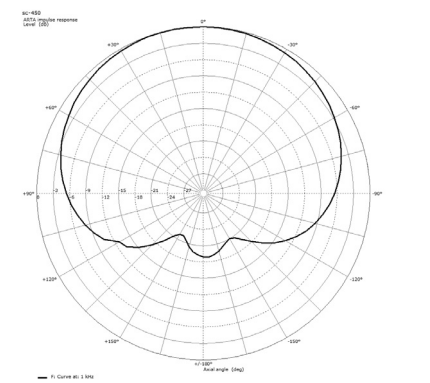
Polar pattern @ 1 kHz
