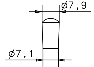
Toggle Switch Knopf toggle switch knob
