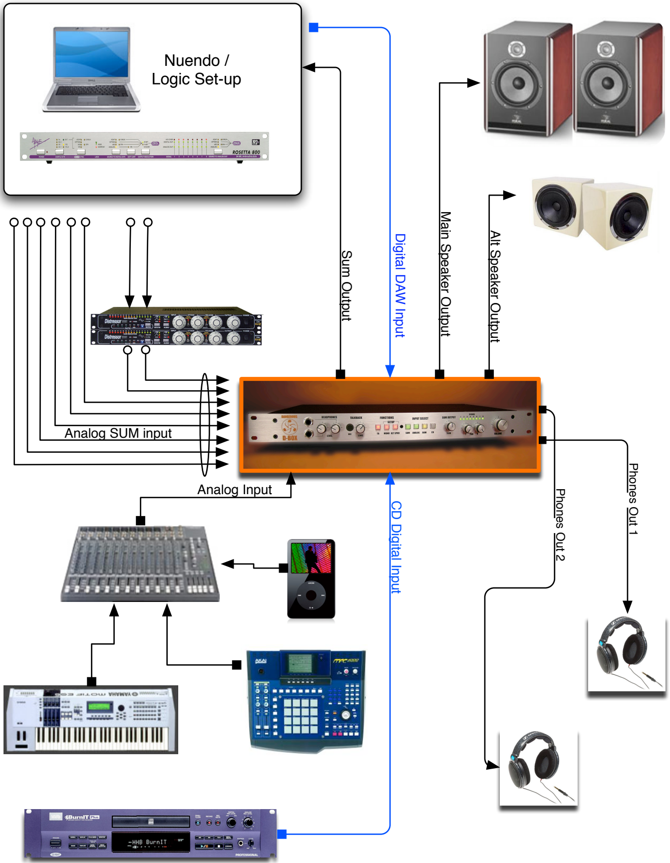
DANGEROUS D-BOX EXTENDED LOGIC OR NUENDO SET-UP
