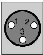
MALE XLR
