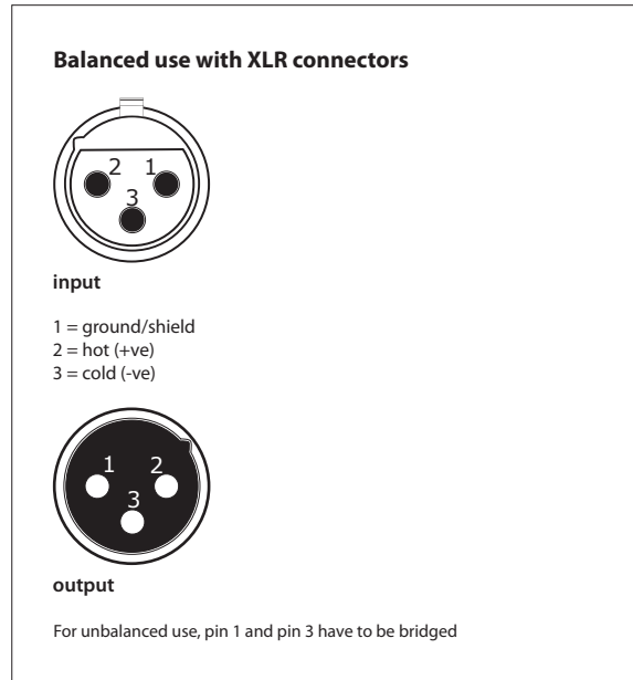
Fig. 5.4: XLR connectors
