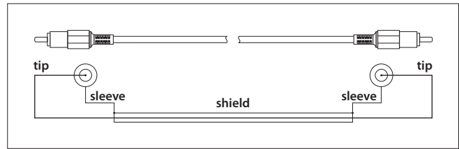
Fig. 5.3: RCA cable
