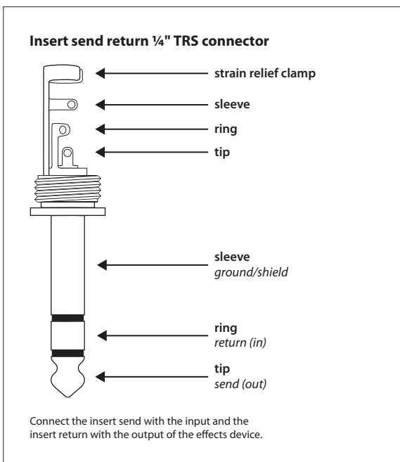
Fig. 5.7: Insert send and return ¼" TRS connector
