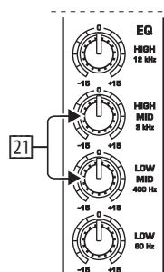
Fig. 2.6: Stereo channel equalizer
