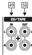
Fig. 2.21: CD/tape connectors
