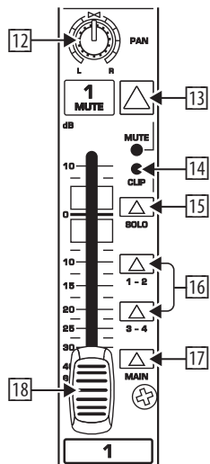
Fig. 2.4: Channel fader, pan control, mute button, etc.
