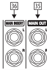
Fig. 2.15: Main out connectors and main insert
