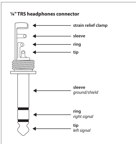
Fig. 5.6: ¼" TRS connector for headphones
