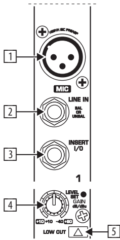
Fig. 2.1: Connectors and controls of the mic/line inputs
