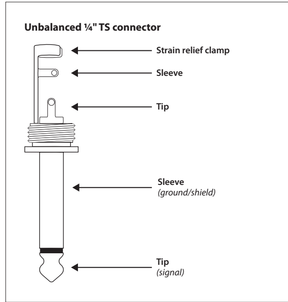
Fig. 5.1: 1/4" TS connector
