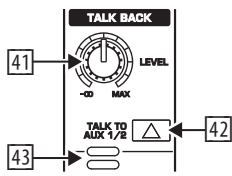
Fig. 2.17: Talkback section
