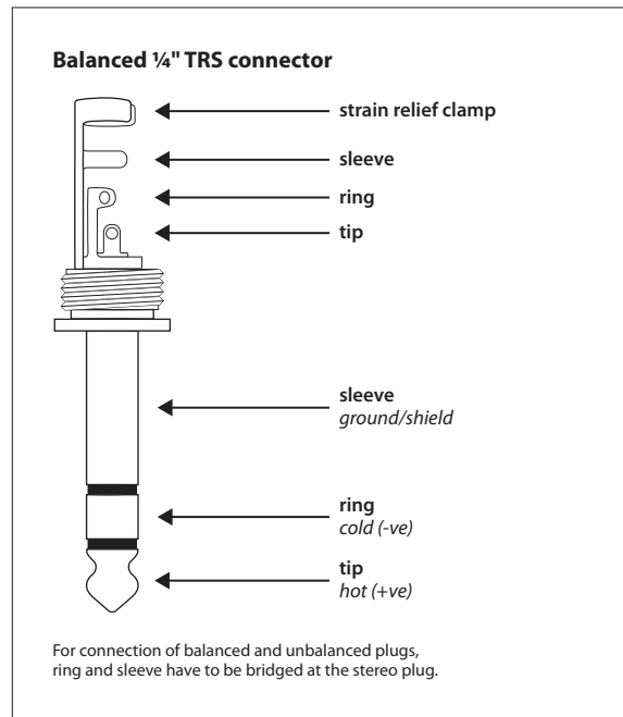
Fig. 5.2: 1/4" TRS connector
