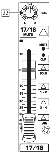
Fig. 2.7: Channel fader, balance control, mute switch, etc.
