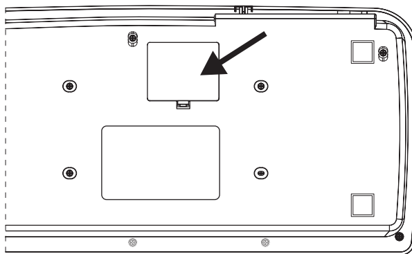
Fig. 1.2: The battery compartment on the bottom side of the UMX.
