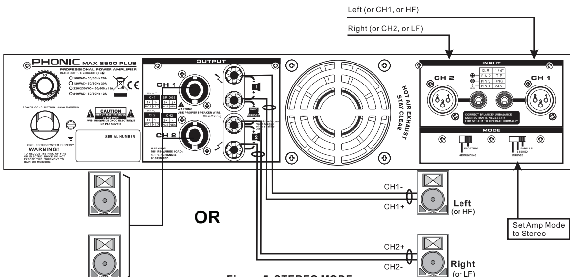
Figure 5 STEREO MODE
