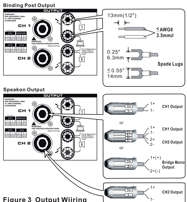
Figure 3 Output Wiring
