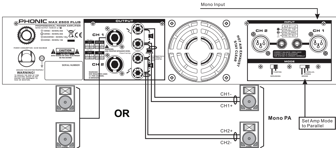
Figure 4 PARALLEL MODE
