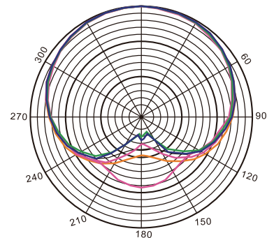
Polar pattern @ 1 kHz
