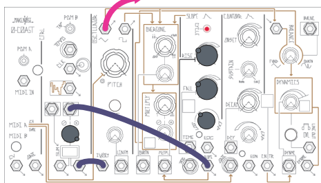
Figure 32: Triangle Wave: Base Frequency (No Control Voltage Applied)
