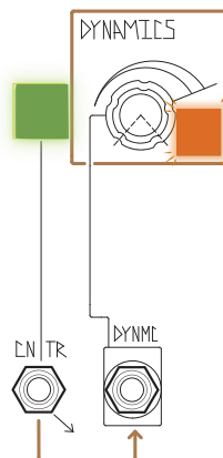
Figure 47: CONTOUR Normalization
