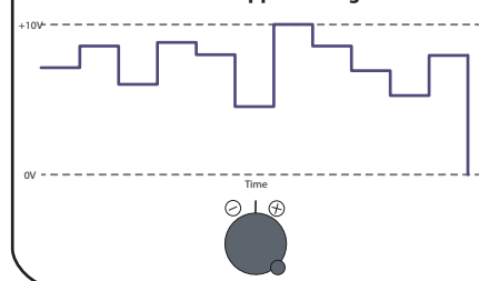
Figure 30: Random Stepped Voltage
