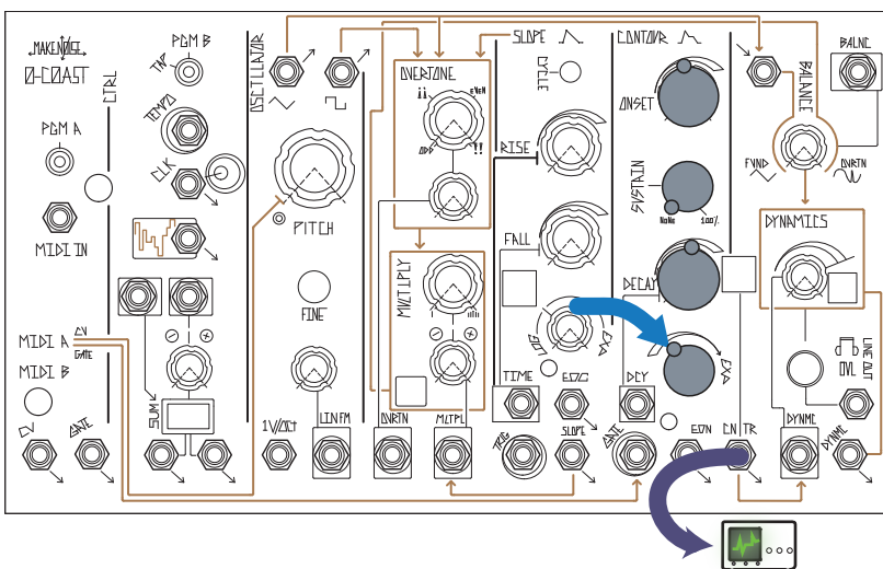
Figure 51: Contour Typical AD Function
