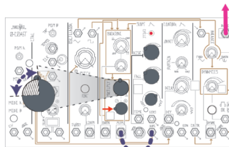
Figure 36: Adding the SLOPE's unipolar voltage to the MULTIPLY Panel Control Offset. The resulting "range" of movement is indicated by the crosshatched area of the MULTIPLY Panel Control.
