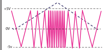
Figure 33: Triangle Wave: Exponential Frequency Modulation
