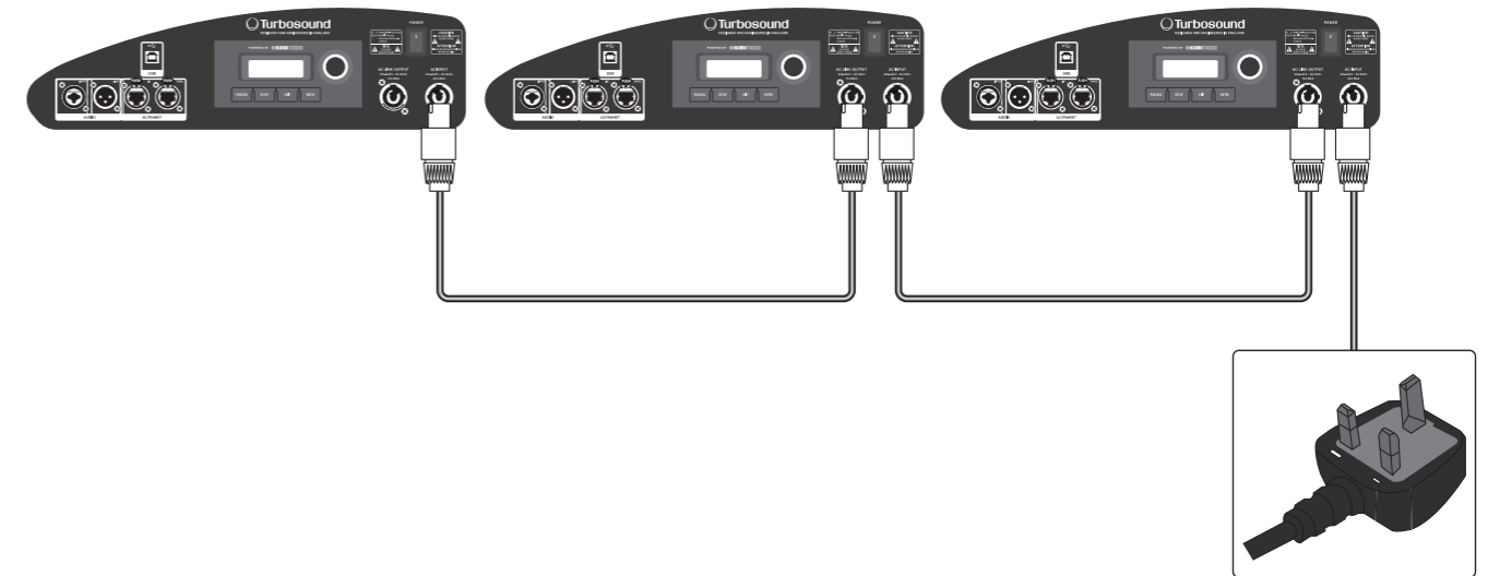
TFM-AN speakers powered in series
