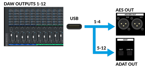
DAW feeds digital outputs mode - AES and ADAT fed from USB. Example given at 44.1/48 kHz
