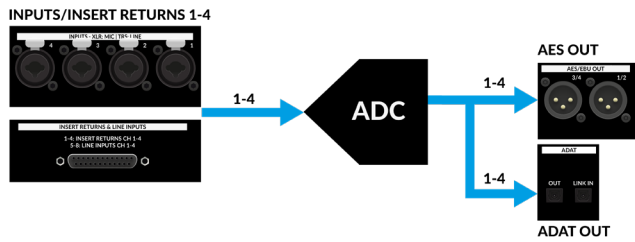
Normal mode - AES and ADAT Outputs fed from A-D converter
