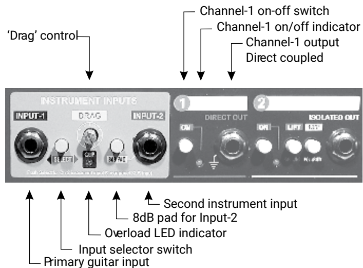
JD7 Instrument inputs, Channel-1 & Channel-2 outputs.
