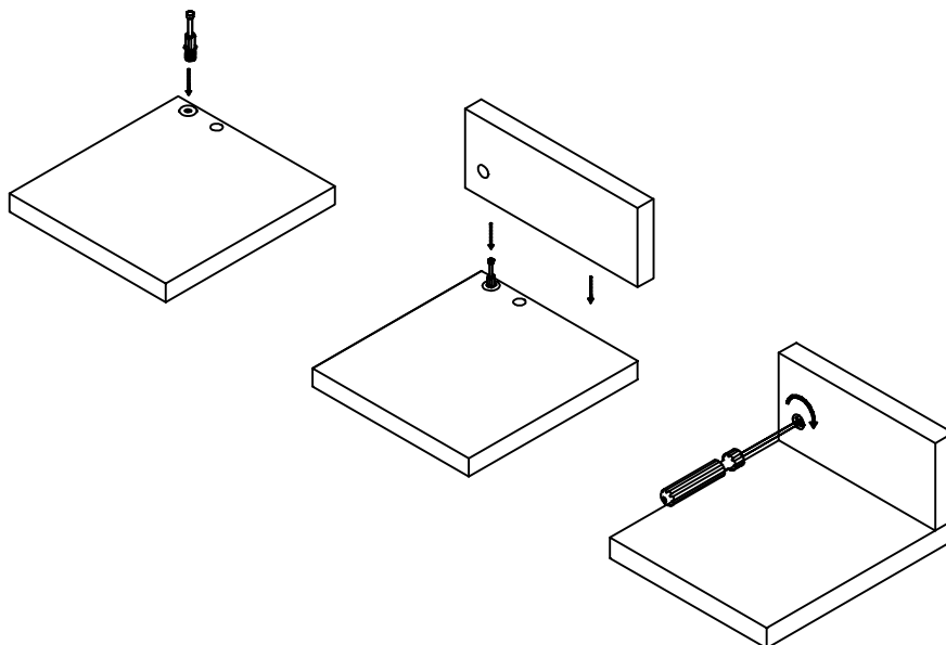
Expanding socket
