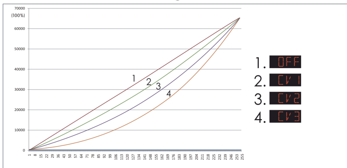
Dimming curves
