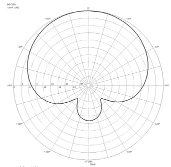
Polar pattern @ 1 kHz
