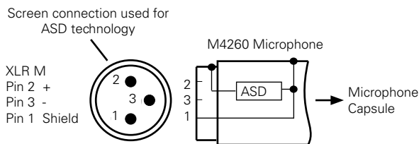
Connection Diagram of Measurement Microphones M4260 and M2210 - Enhanced Performance
