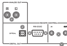
CD-C600RK Rear Panel
