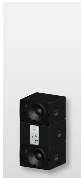
2 x G Sub 1501 dp+ / G Sub 1501 Cardioid set-up.
