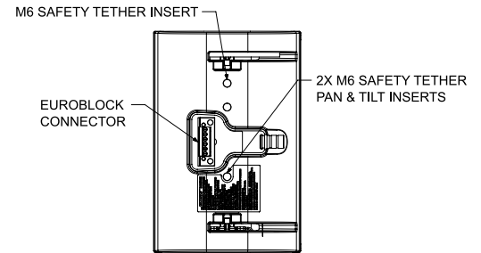
Rear View BRACKET/INPUT COVER REMOVED FOR CLARITY
