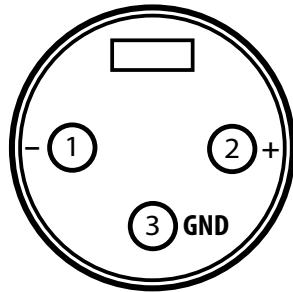
XLR plug viewed from above
