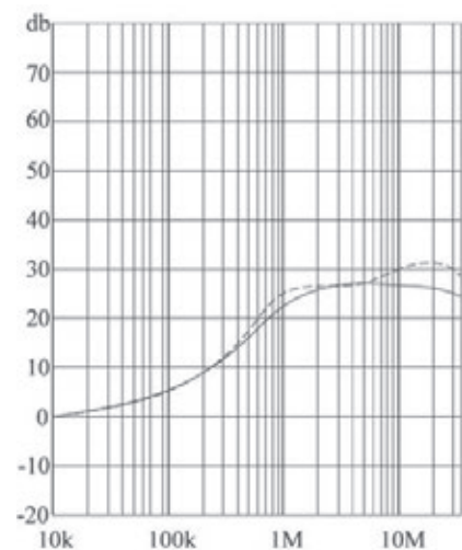
Insertion loss in 50 Ω System ----- Differential mode / Symmetrical (L-L) ————— Common mode / Asymmetrical (L-G)
