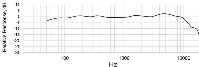
KSM313/NE Frequency Response (Rear)
