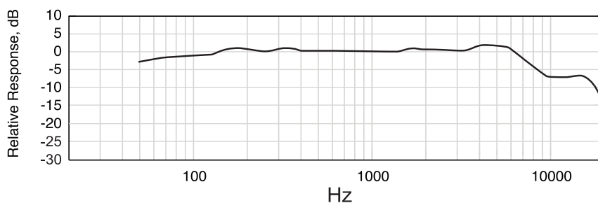
KSM313/NE Frequency Response (Front)
